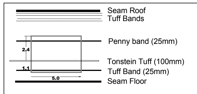
Fig. 4 Horizon control for typical ground
